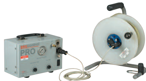
geocontrol PRO™ with optional draw-down control for low flow sampling
