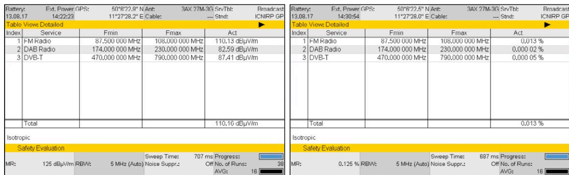
Figure 2.18: Automatic immission measurement of sound radio and TV signals in Safety Evaluation mode (left: absolute display; right: relative display as a percentage of the limit value). Measured in AUTO mode, i.e. the predefined RBW values in the service table are ignored and the device automatically selects a fixed RBW (5 MHz in this case).
