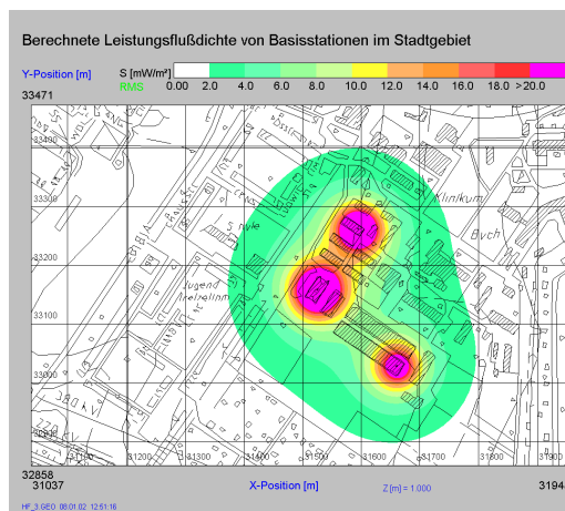
Fig. 3. Power flux density in an urban area
