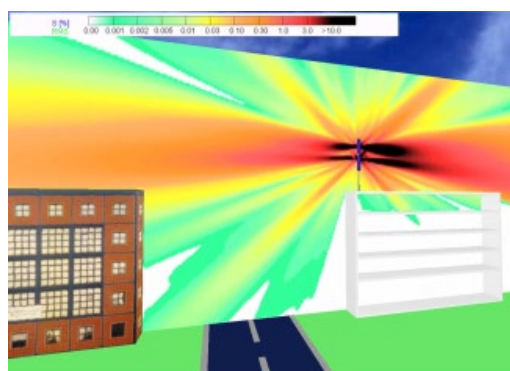
Fig. 2. Mobile telecoms antenna on a building
