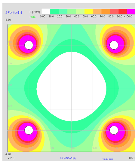
Fig. 6. Four-conductor bundle surface field strength
