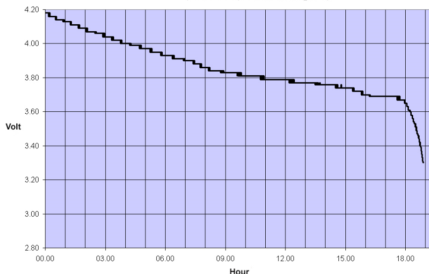
Fig. 2-3 EHP-200A/AC Battery Discharging
