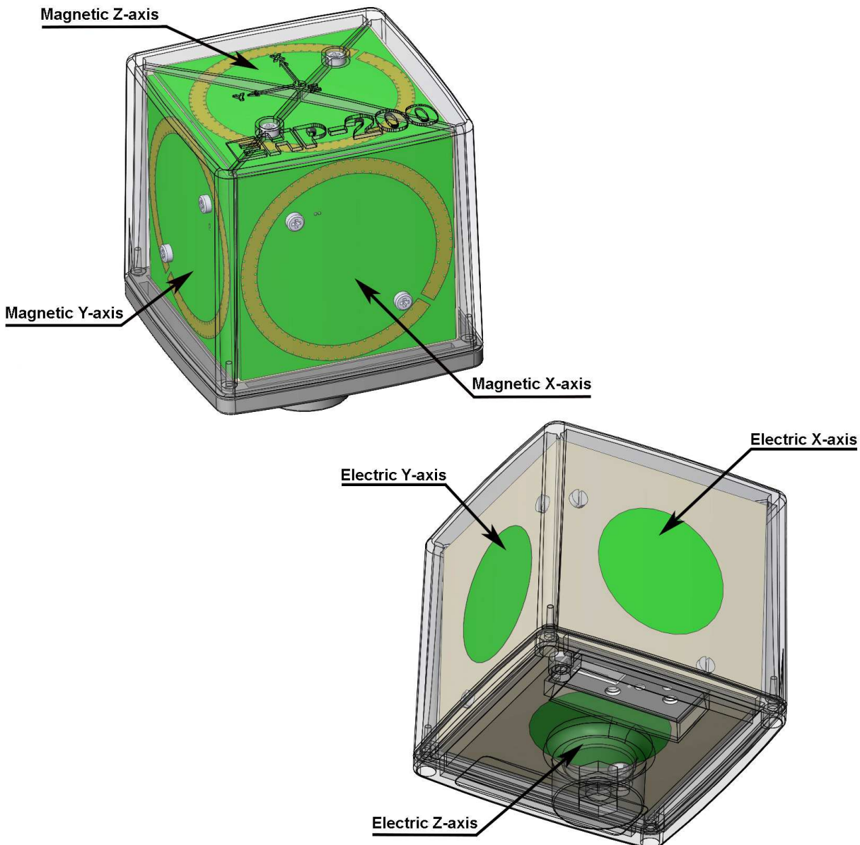
Fig. 1-4 EHP-200A/EHP-200AC axes
