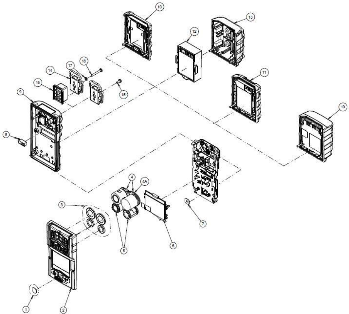
Figure 8.1 Instrument diagram
