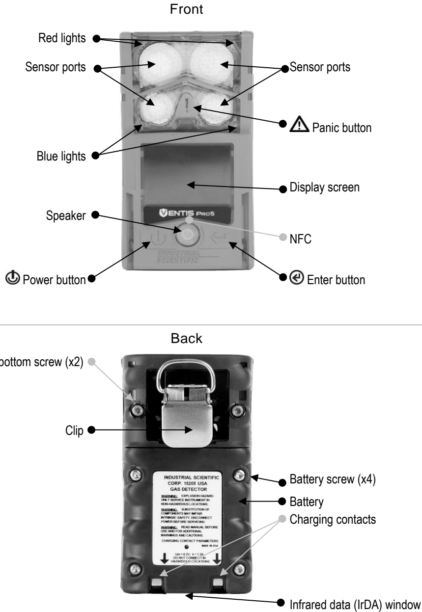
Figure 3.1.A Hardware overview diffusion instrument
