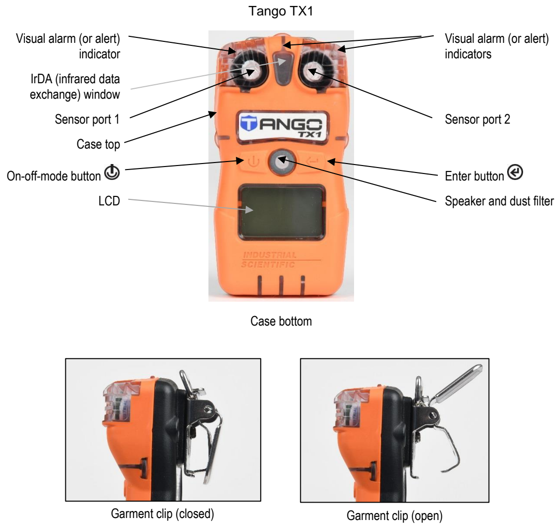
Figure 3.1 Hardware overview
