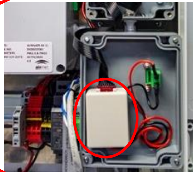
Figure 6-17 – Pump Internal
