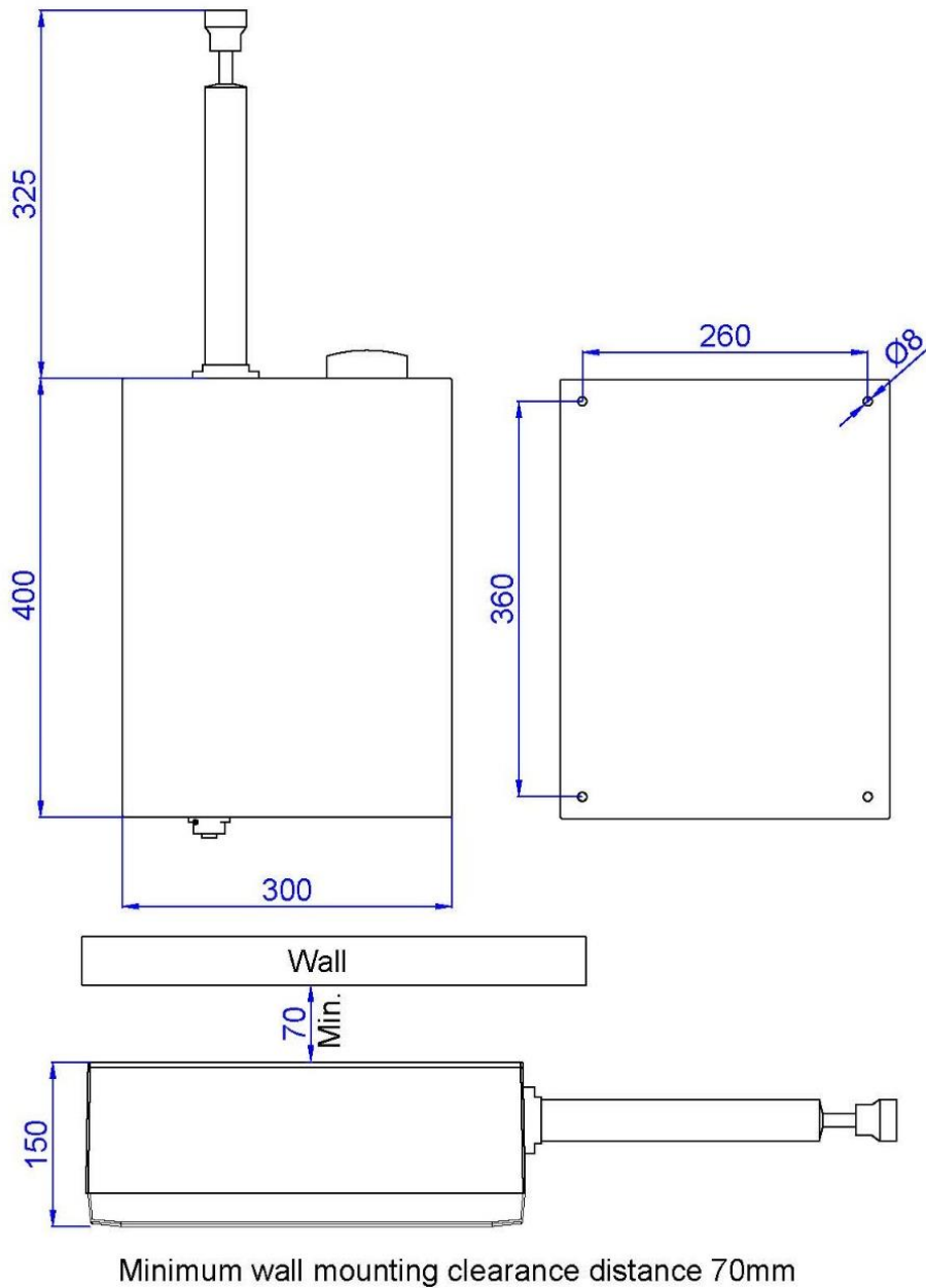
Figure 4-3 – External and Mounting-Point Dimensions (mm)
