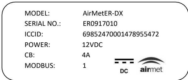
Figure 3-1 – Monitor Product Label Example
