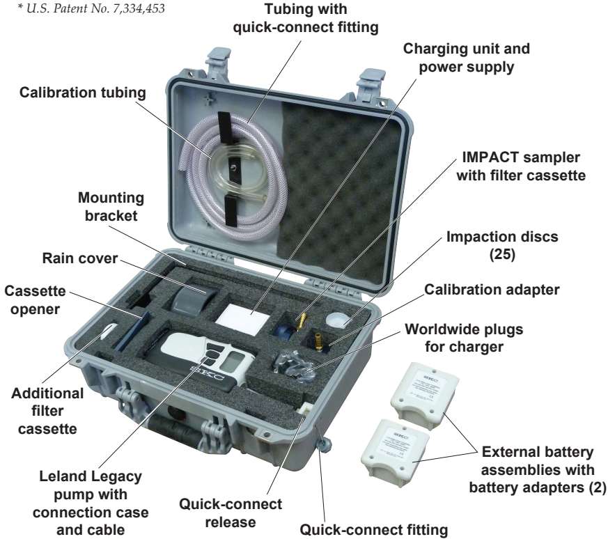
The SKC DPS System includes a Leland Legacy Sample Pump with connection case and charger (100-240 V), IMPACT sampling head, 2 filter cassettes, calibration adapter, rain cover for sampling head, 25 disposable impaction discs, filter cassette opener, tubing with quick-connect fitting, and mounting bracket in a heavy-duty lockable carry case. Two external battery assemblies with adapters are packaged separately.
