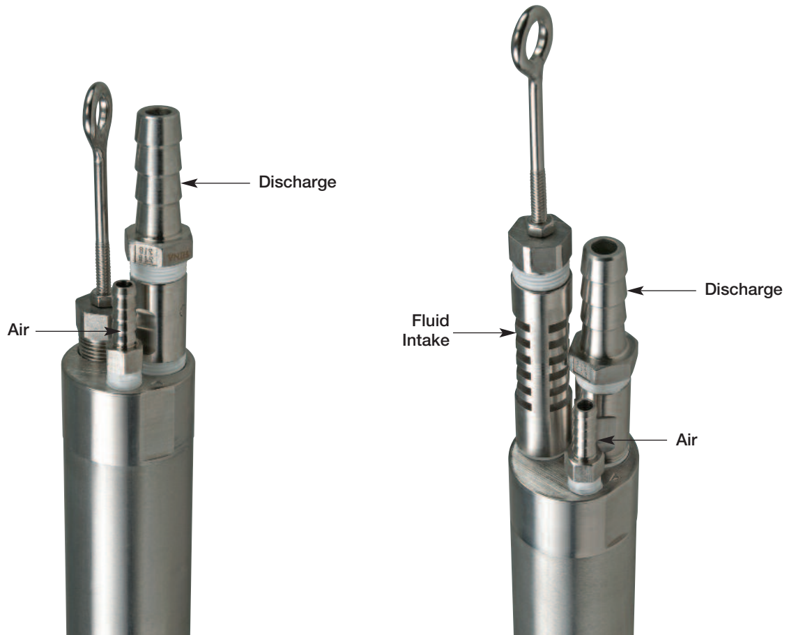
Figure 1 1.66" Reclaimer Bottom Fill
