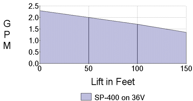
Pump Curve
