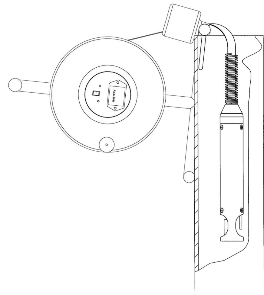
Figure 2-1: Reel frame on well casing.
