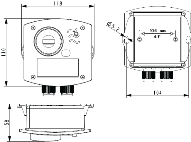
Figure 2: OLCT 10N dimensions (in millimeters)
