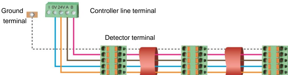
Figure 3: Schematic for connecting modules on a MX 43 line
