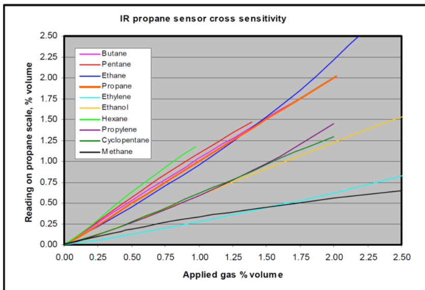
Figure F - 2 Cross-sensitivity chart for iTRAN5-2 Propane IR Sensor
