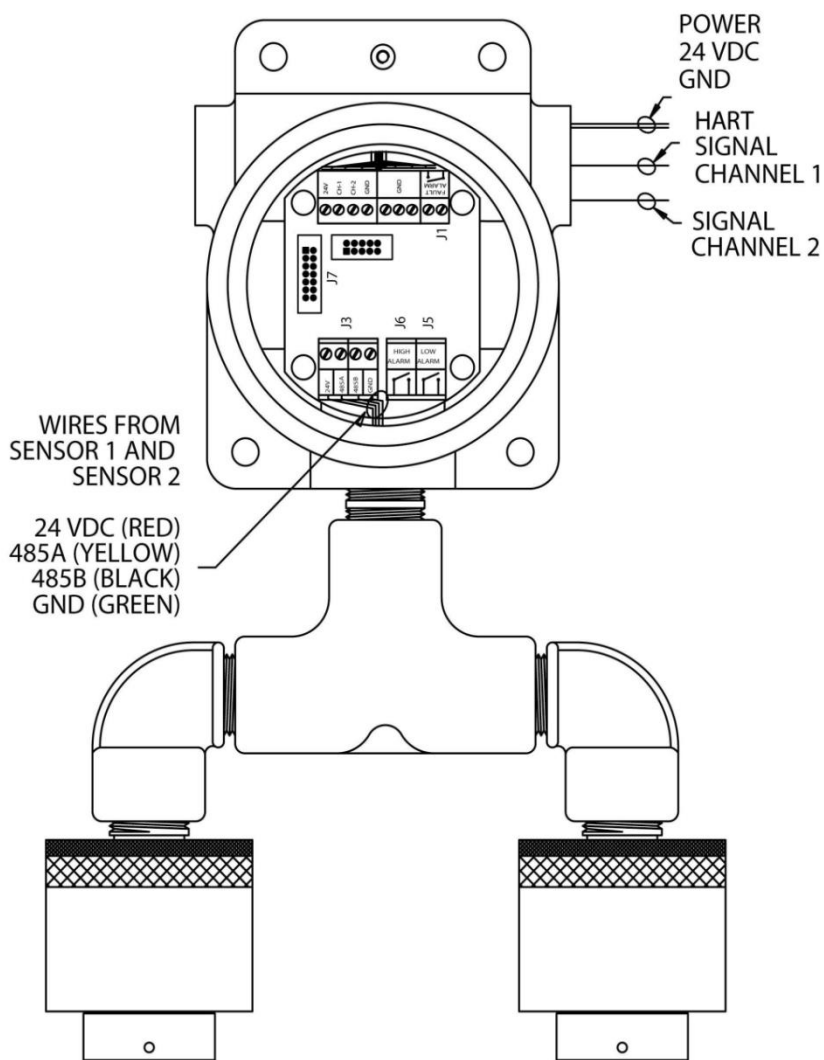
Figure A - 5 Wiring Diagram of Dual Sensor HART Supported TRANS-2
