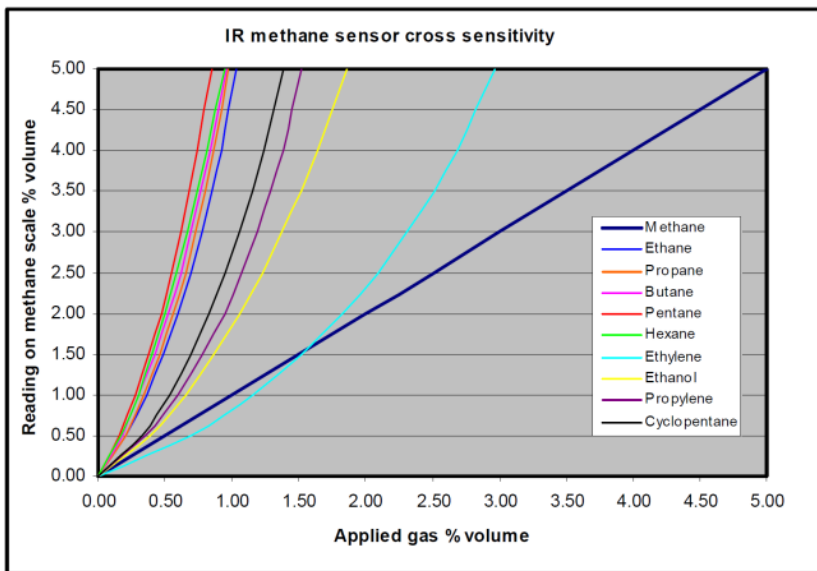
Figure F - 1 Cross-sensitivity chart for TRANS-2 methane IR Sensor
