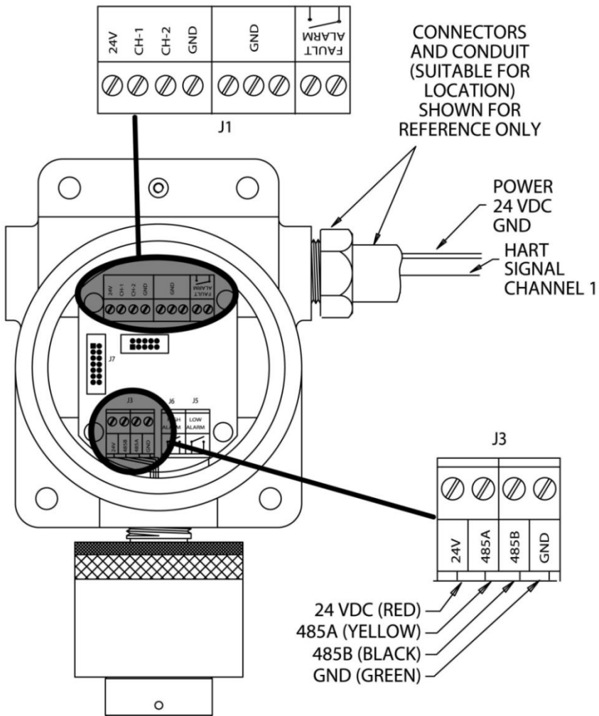
Figure A - 4 Wiring Diagram of Single Sensor HART Supported itTRANS-2
