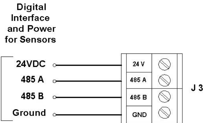
Figure 4-3 Sensor Connector J3 on the ITRANS-2
