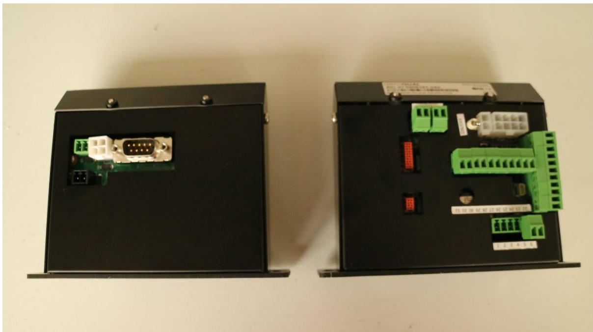
Figure 0-14 Left IO module for the 82850 optical module, note that the fiber span switch is no longer used, Right IO module for the 80180 optical module
