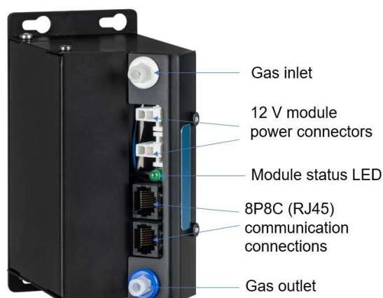
Figure 0-4 Gas sensor module with key components labelled
