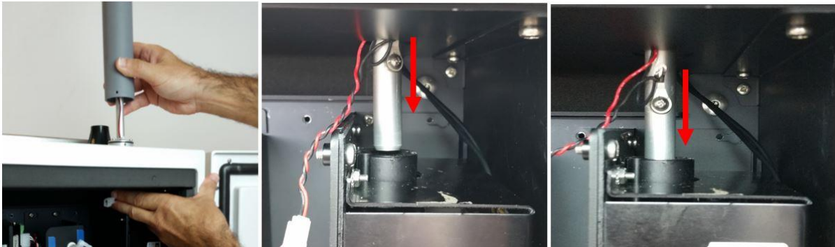
Figure 0-7 Gently feed in the power cable. The aluminum tube must push all the way in to the PM module.
