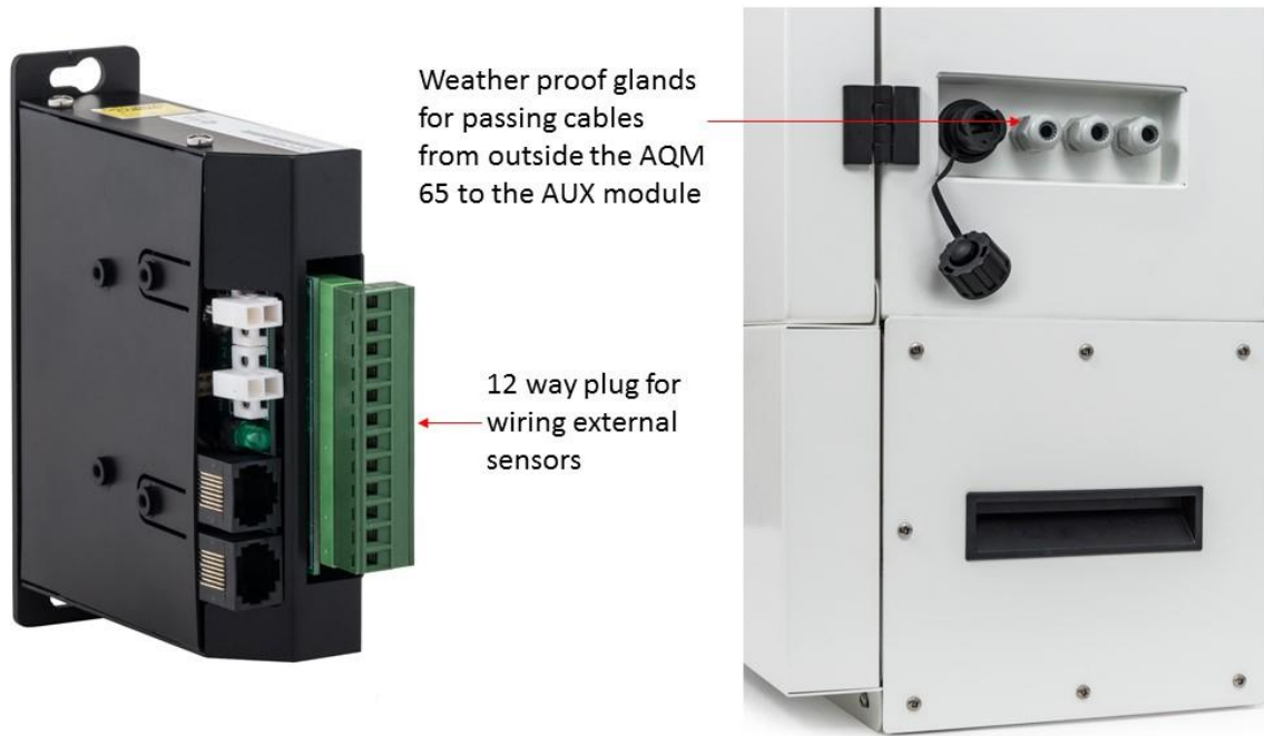
Figure 0-19 The external sensors are connected to the green plug on the Aux module. The cable passes through water proof glands on the right wall of the AQM 65
