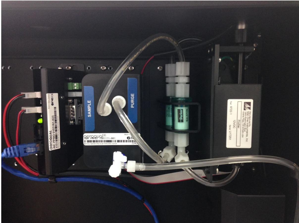
Figure 0-16 The Particle Profiler uses three modules: a) the optical module on the far right, b) the pump module in the middle, c) the electronics module on the left. The image above is the arrangement prior to July / August 2018.
