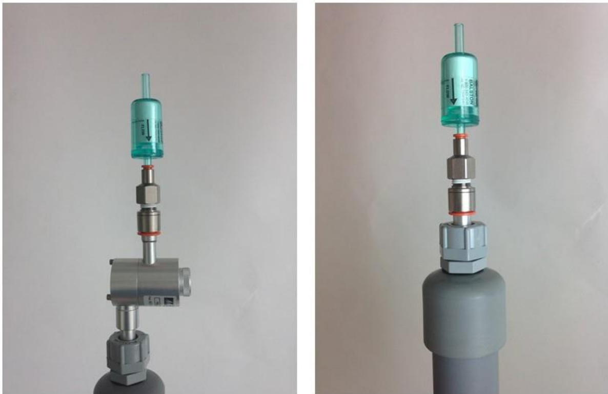
Figure 0-22 The zero filter is fitted above the cyclone for a Particle Monitor (left) and directly on the inlet for a Particle Profiler (right)
