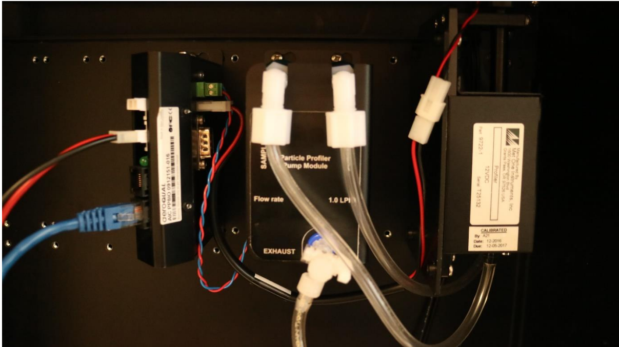
Figure 0-17 An update to the pump module with the filters installed inside the pump module
